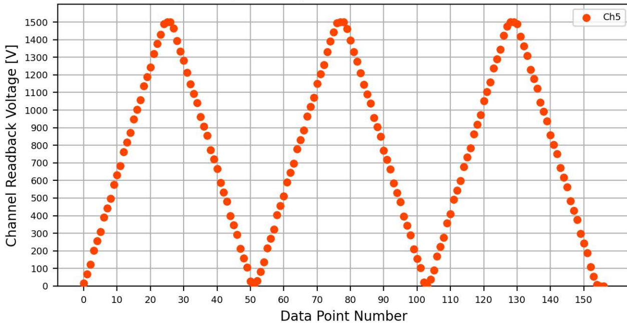
Voltage Ramp Test (Python) Bd #776, Slot #3, Ch #5
