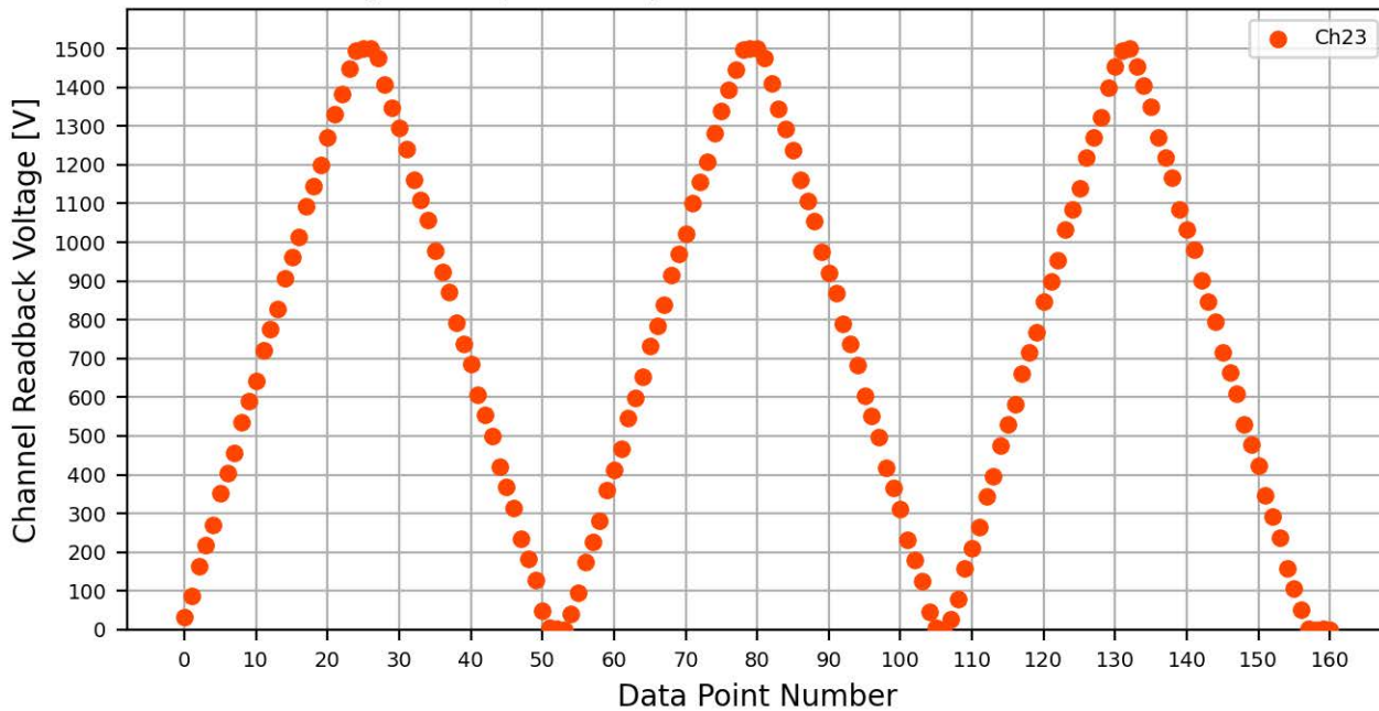
Voltage Ramp Test (Python) Bd #776, Slot #3, Ch #23
