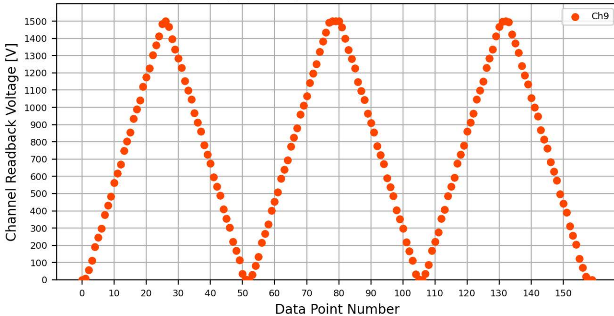
Voltage Ramp Test (Python) Bd #776, Slot #3, Ch #9
