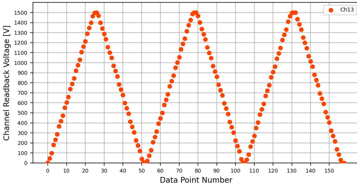
Voltage Ramp Test (Python) Bd #776, Slot #3, Ch #13
