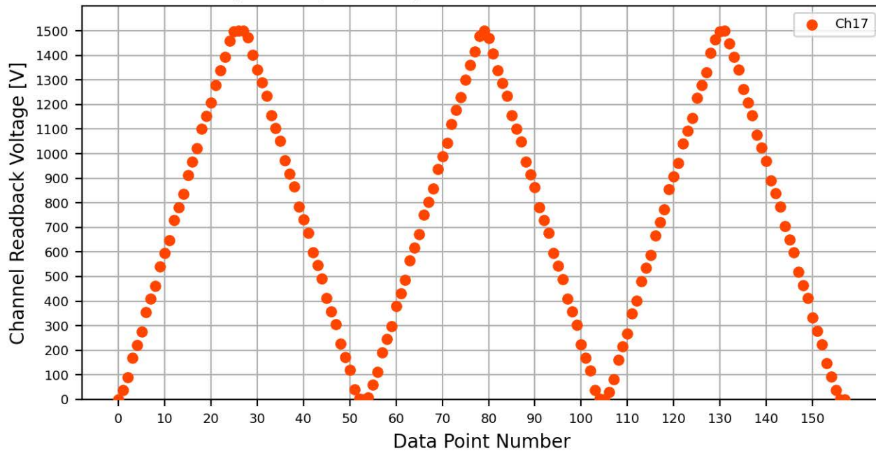
Voltage Ramp Test (Python) Bd #776, Slot #3, Ch #17
