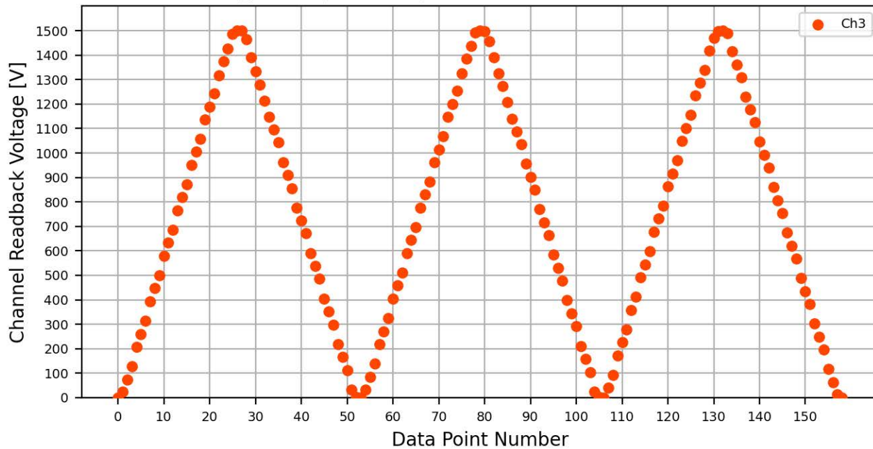
Voltage Ramp Test (Python) Bd #776, Slot #3, Ch #3
