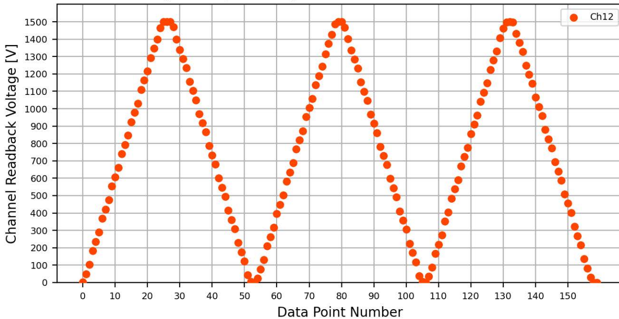
Voltage Ramp Test (Python) Bd #776, Slot #3, Ch #12
