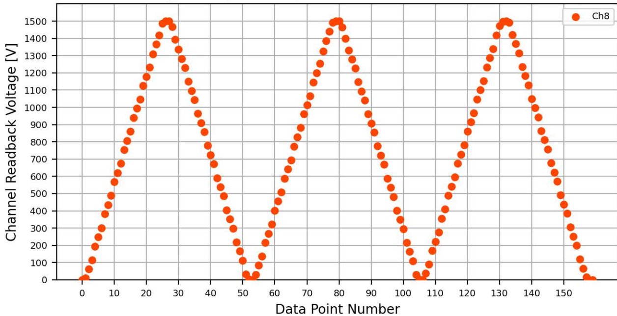
Voltage Ramp Test (Python) Bd #776, Slot #3, Ch #8
