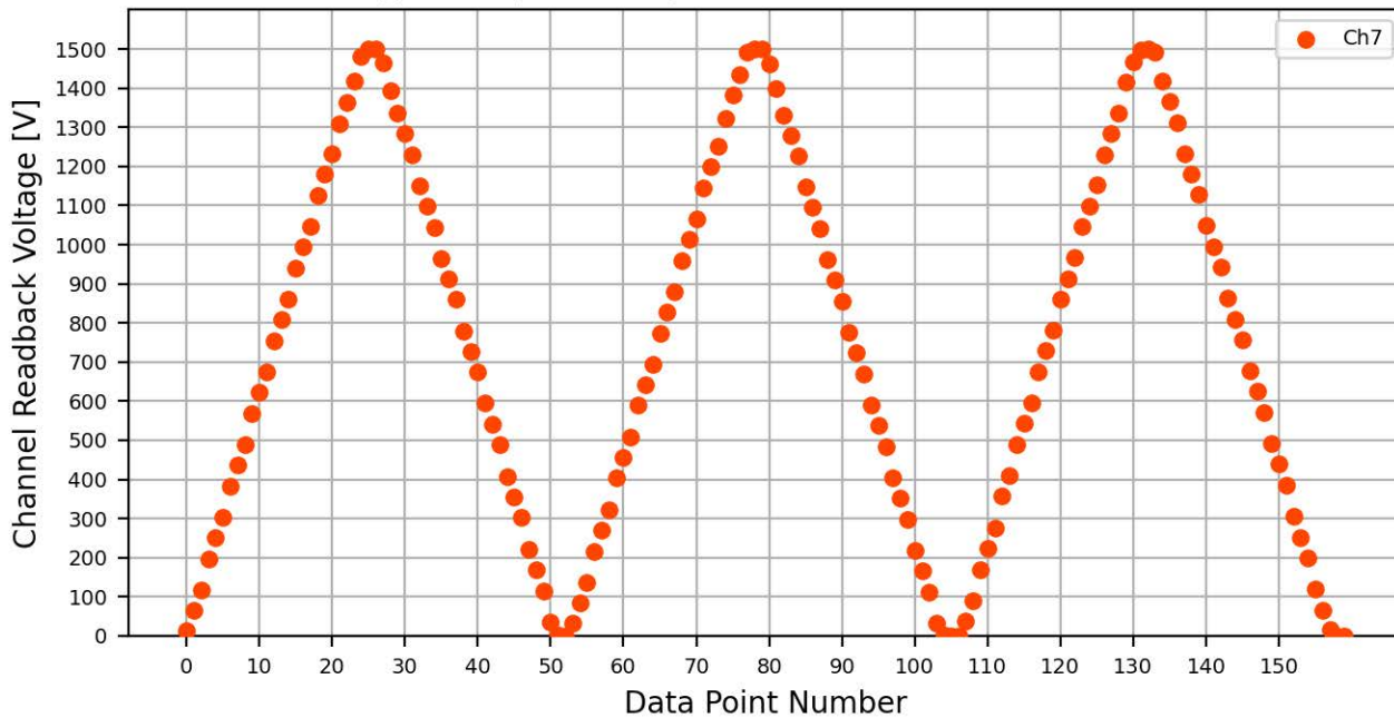
Voltage Ramp Test (Python) Bd #776, Slot #3, Ch #7
