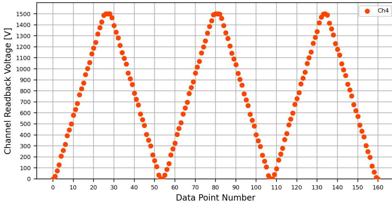
Voltage Ramp Test (Python) Bd #776, Slot #3, Ch #4
