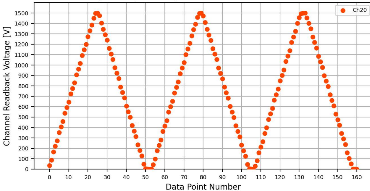
Voltage Ramp Test (Python) Bd #776, Slot #3, Ch #20
