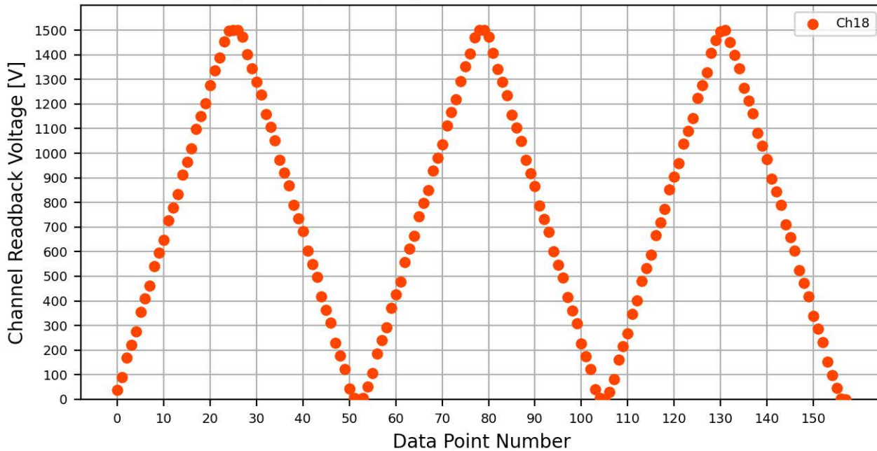
Voltage Ramp Test (Python) Bd #776, Slot #3, Ch #18
