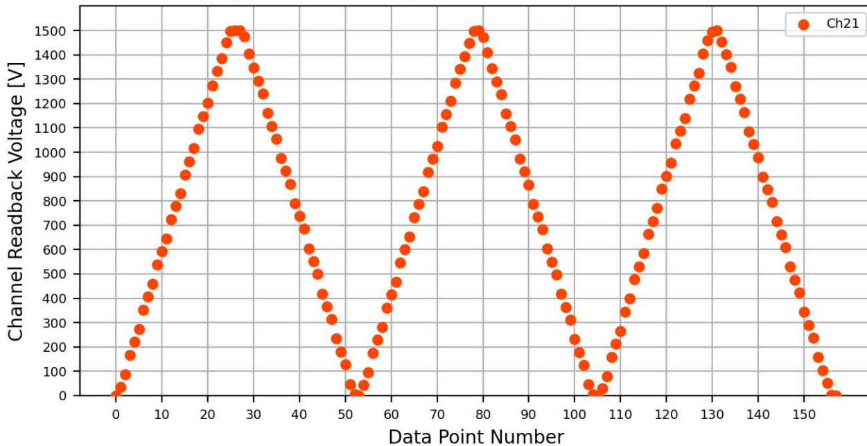
Voltage Ramp Test (Python) Bd #776, Slot #3, Ch #21
