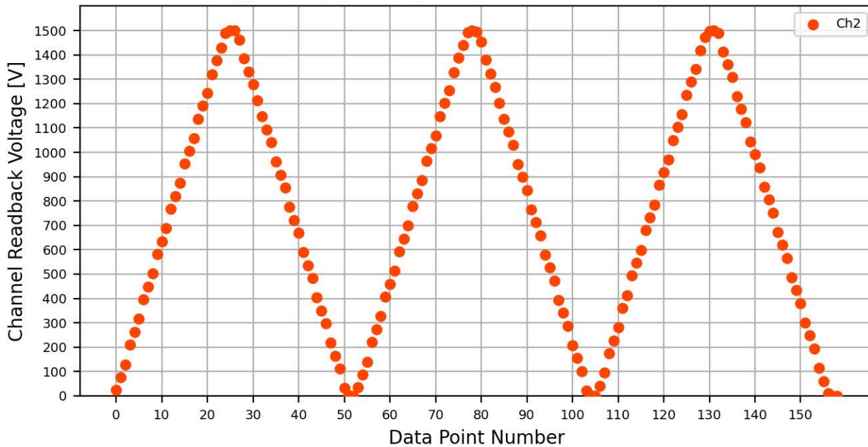
Voltage Ramp Test (Python) Bd #776, Slot #3, Ch #2
