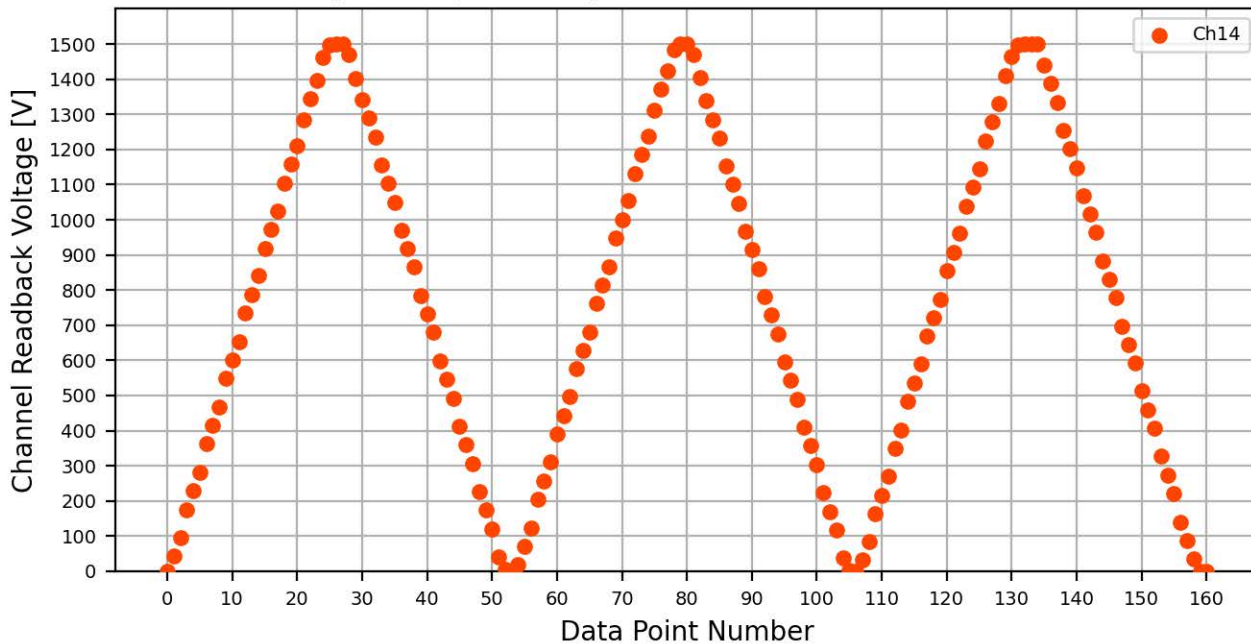
Voltage Ramp Test (Python) Bd #776, Slot #3, Ch #14
