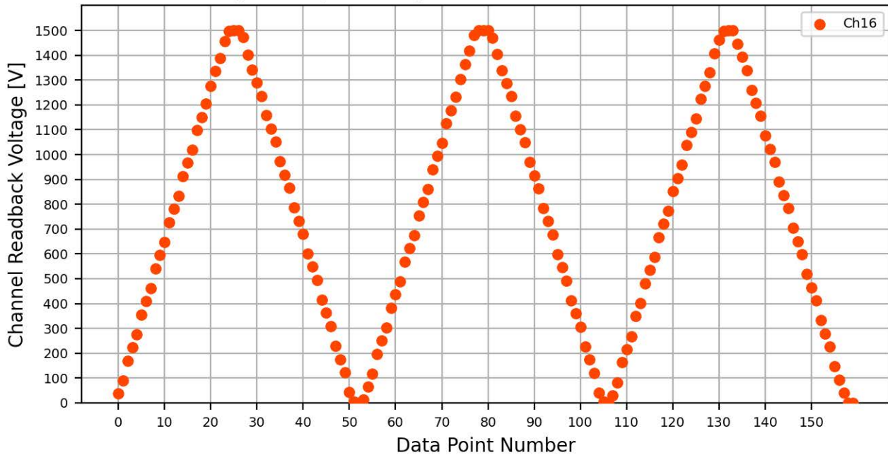
Voltage Ramp Test (Python) Bd #776, Slot #3, Ch #16
