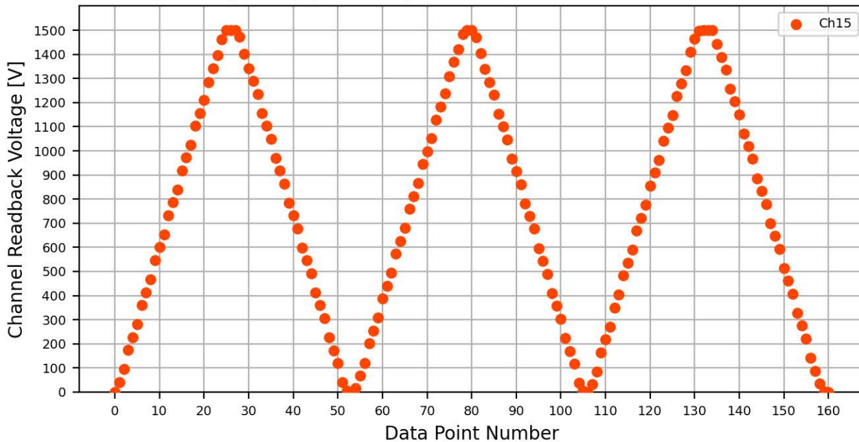
Voltage Ramp Test (Python) Bd #776, Slot #3, Ch #15
