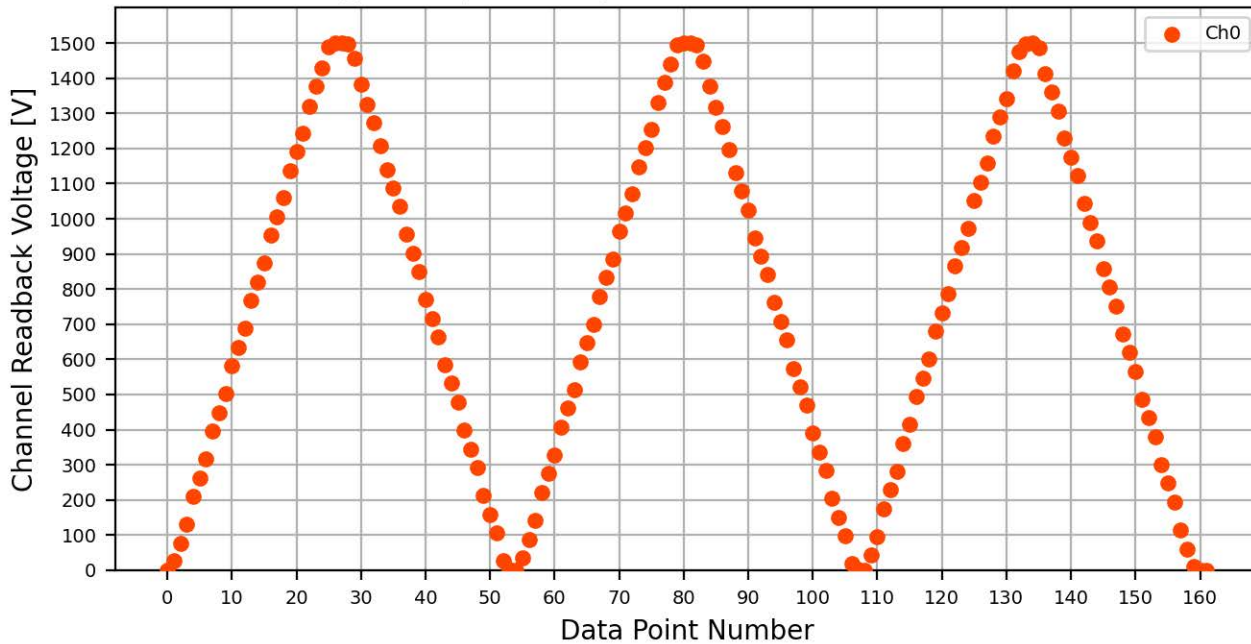
Voltage Ramp Test (Python) Bd #776, Slot #3, Ch #0
