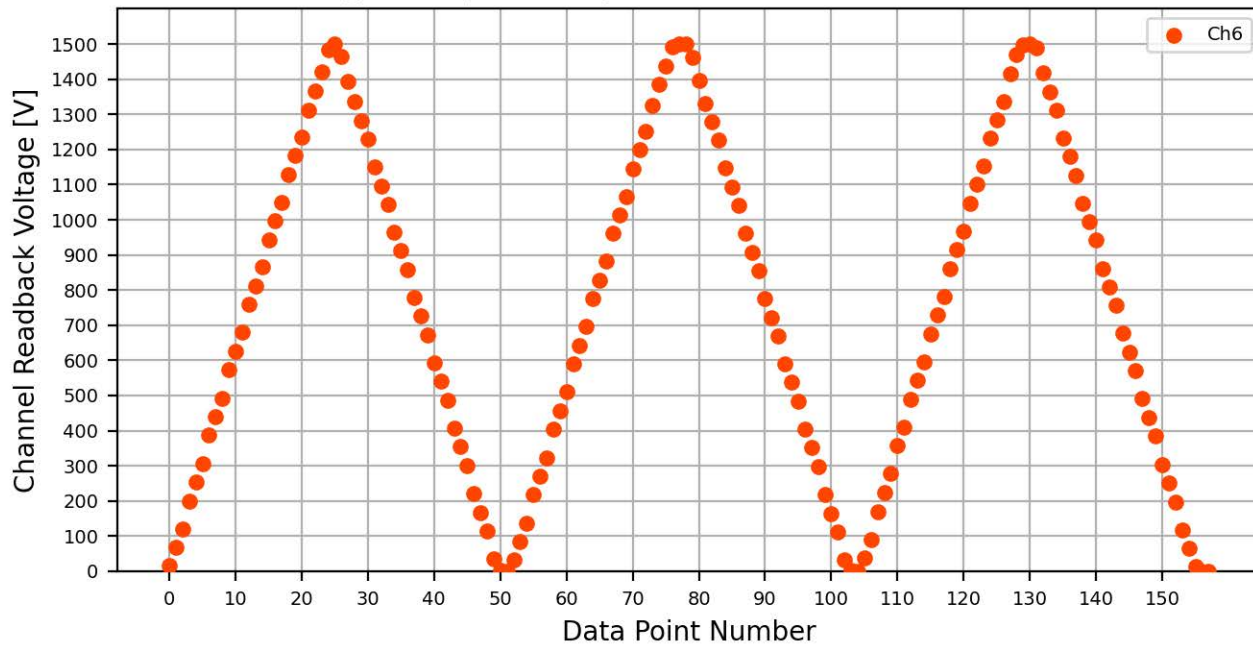
Voltage Ramp Test (Python) Bd #776, Slot #3, Ch #6
