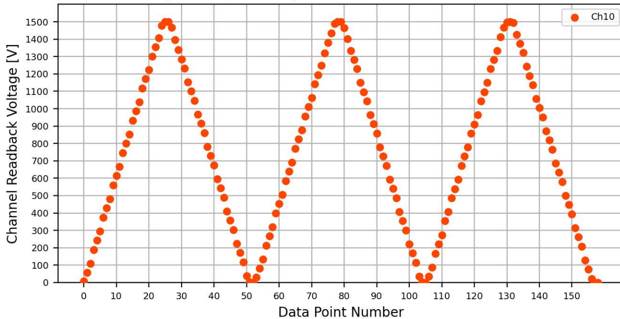
Voltage Ramp Test (Python) Bd #776, Slot #3, Ch #10
