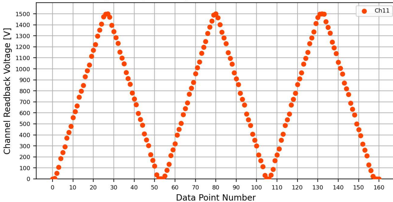
Voltage Ramp Test (Python) Bd #776, Slot #3, Ch #11
