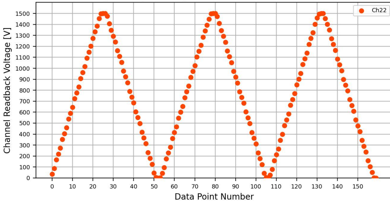
Voltage Ramp Test (Python) Bd #776, Slot #3, Ch #22
