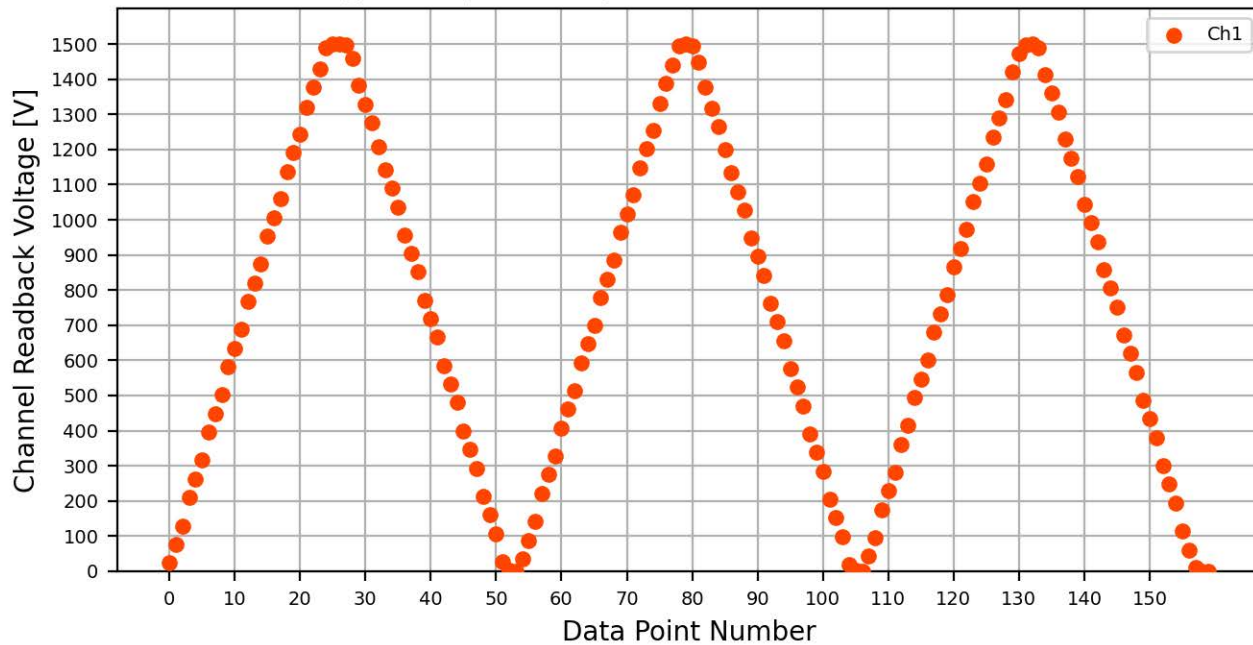
Voltage Ramp Test (Python) Bd #776, Slot #3, Ch #1
